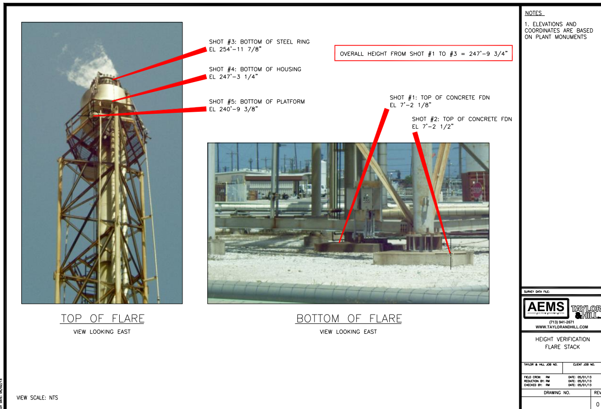
Figure 1: Final CAD drawing submitted to the client shows the elevations requested in a photographic manner
